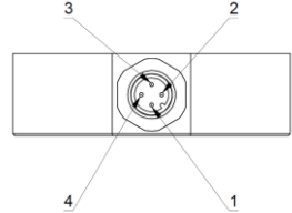
M12 Pinbelegung M12 pin assignment
